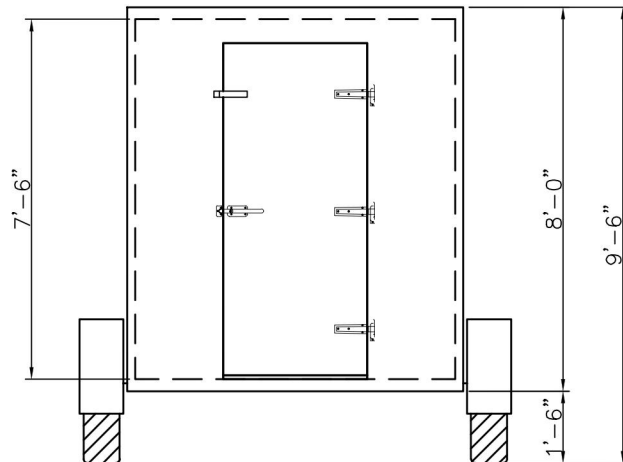
ELEVATION VIEW
