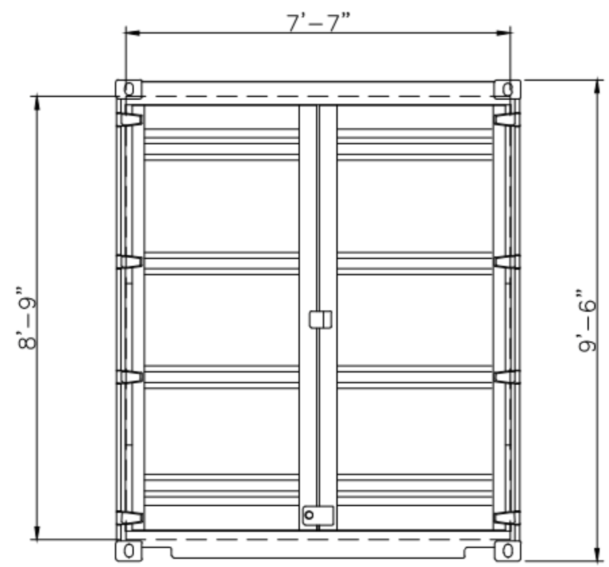
ELEVATION VIEW
