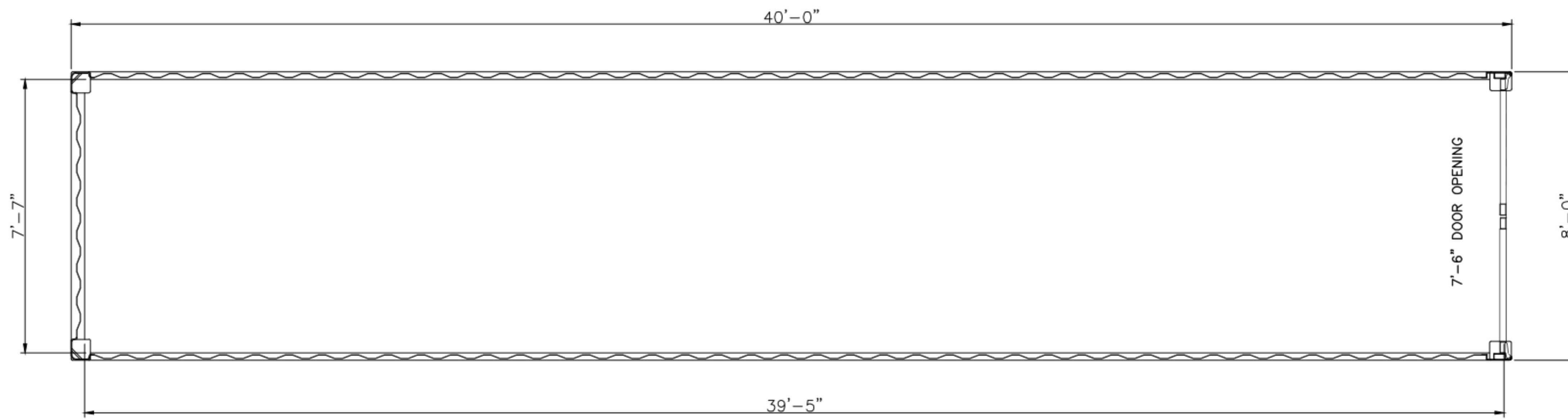
PLAN VIEW
