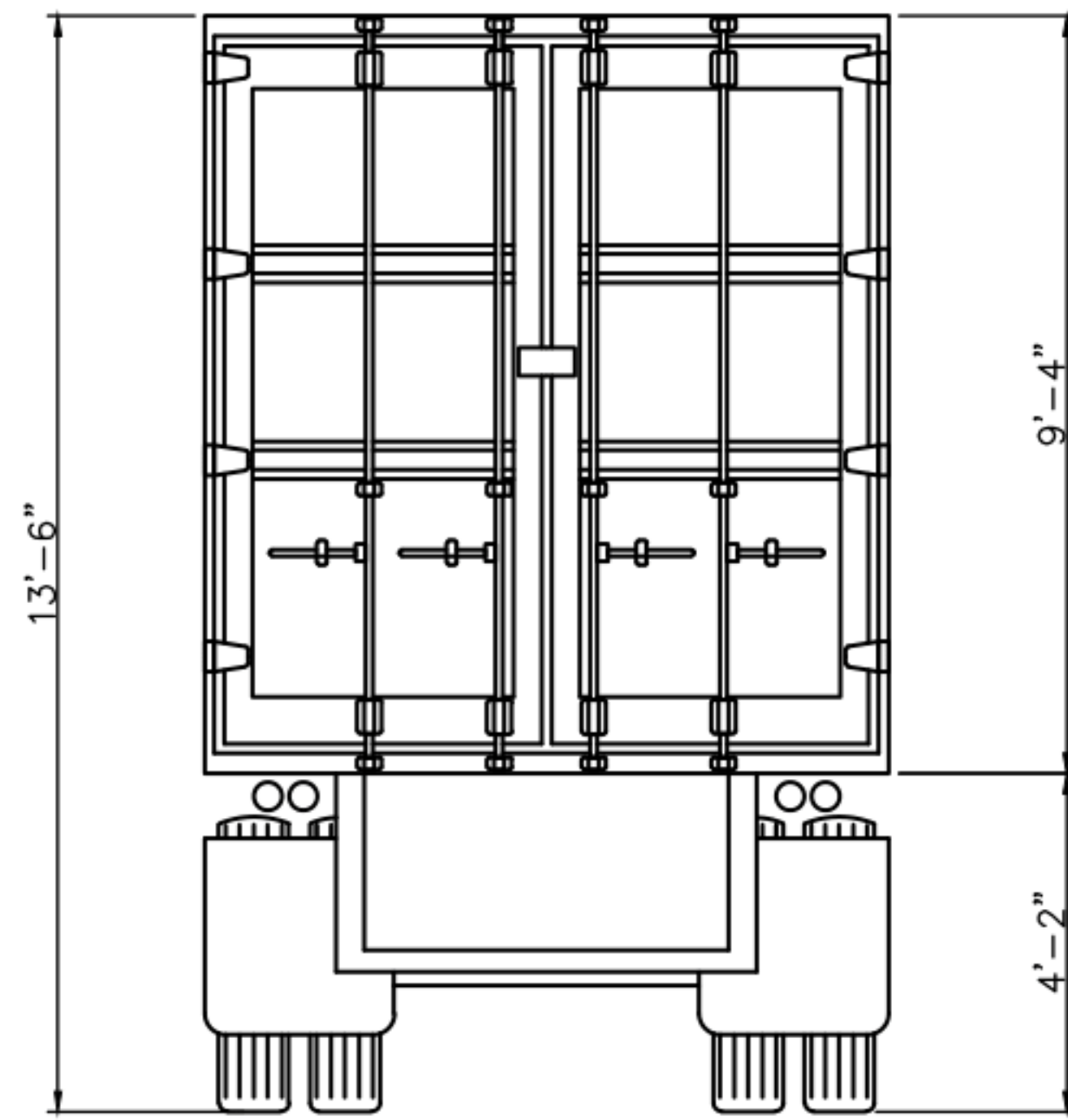
ELEVATION VIEW
